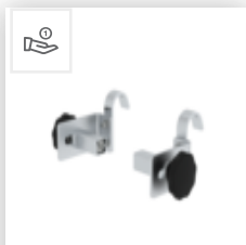
Order no.: 019310 Ladder head protection, rung and step hole \varnothing 36 mm
